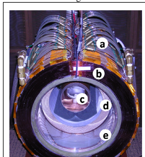
Figure 1: PMRI scanner (a) water cooling (b) 33-cm bore readout magnet (c) resonator (d) 20-cm bore polarizing magnet (e) 3-axis gradient coil set
