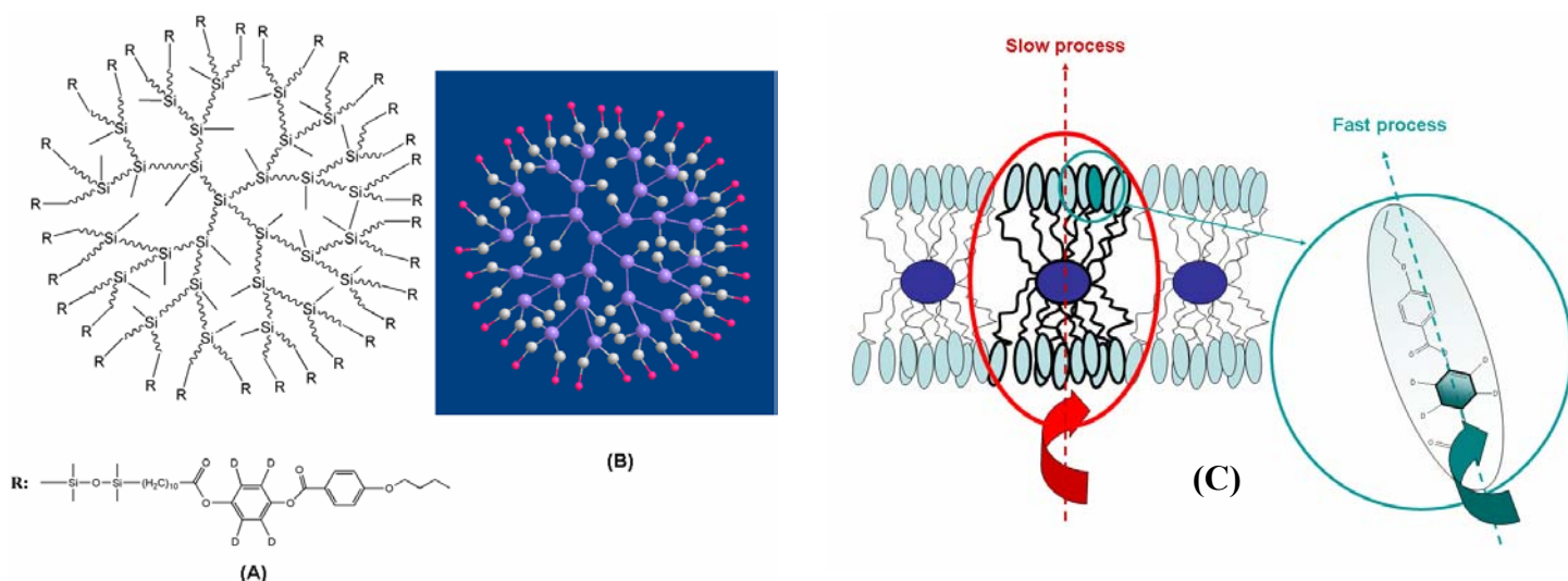
Scheme 1: (A) Molecular structure of the LC dendrimer G-3(Und-R) 32 and its lateral group R; (B) dendrimer in the isotropic phase; (C) two main motional contributions to the ^2\text{H} NMR relaxation.
