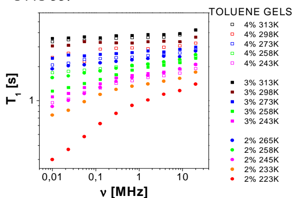
Figure 2. Frequency dependence of the proton spin-lattice relaxation time of toluene in 1,2-O-(1-ethylpropylidene)- \alpha -D-glucofuranose gel.
