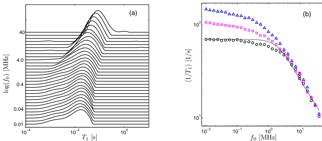
FIG. 1: (a) Evolution of the distribution of T_1 relaxation for a deasphalted crude oil. (b) Dispersion of mean relaxation rates for the deasphalted oil (black circles) and for that same oil with different amounts of dissolved asphaltene (squares and triangles).
