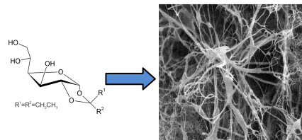
Figure 1. A schematic structure of studied gelator and SEM image of its 3 wt % benzene gel.
