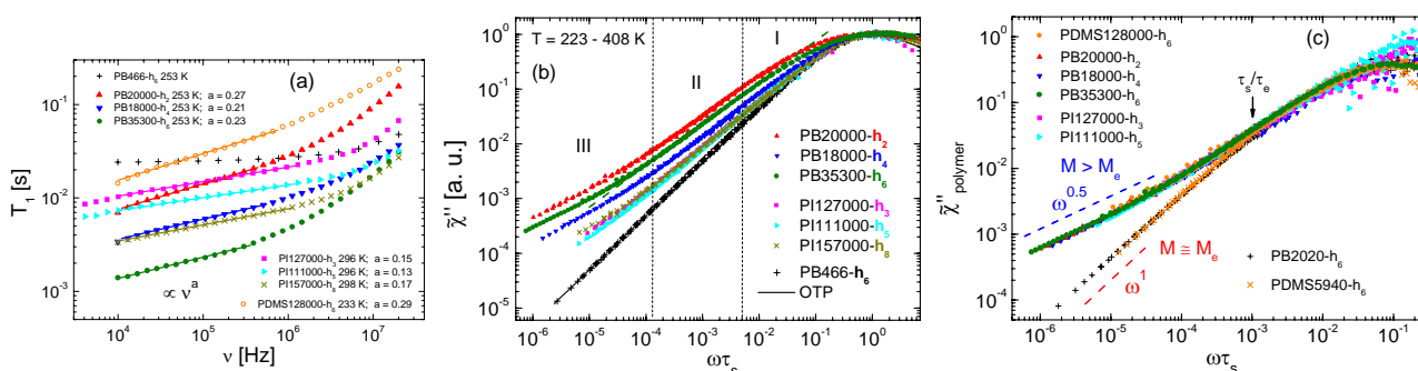
Fig. 1. (a) T_1 -Dispersion data for various polymers. (b) Corresponding susceptibility master curves. (c) Universal “polymer spectra” after subtracting glassy spectrum.
