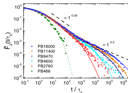
Fig. 2. Dipolar correlation function showing the crossover from Rouse to entanglement dynamics, the latter being characterized by a bimodal shape.
