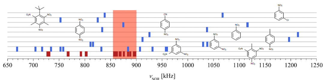
Fig.1. The sensitivity of ^{14}\text{N} NQR on the chemical and structural environment is demonstrated by the NQR frequencies of -\text{NO}_2 groups in some of TNT related compounds. The rows from top to bottom contain spectra for: m-chloronitrobenzene, 2,4,6-trinitro-1-t-butyl-3,5-dimethylbenzene, p-nitrobenzonitrile, nitrobenzene, p-nitrotoluene, m-dinitrobenzene, trinitrobenzene, and trinitrotoluene (orthorhombic and monoclinic). Only the \nu_+ and \nu_- frequencies are shown. The shaded region shows the part of the spectrum that overlaps with the TNT \nu_+ frequencies.
