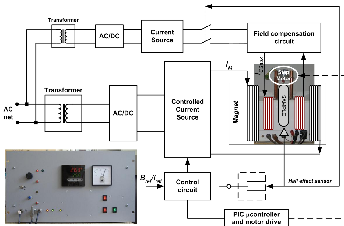
Figure 1 - Main blocks of the desktop FFC relaxometer
