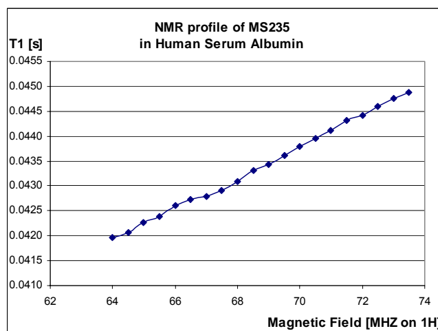
Fig. 2 NMRD profile of MS235 contrast agent in Human Serum Albumin
