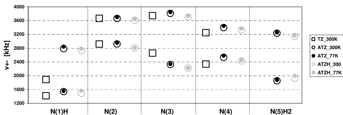
Fig.2. Assignment and comparison of the corresponding \nu_+ and \nu_- ^{14}\text{N} NQR pairs, suitably combined from 1H-tetrazole (TZ, published data ii ), 5-aminotetrazole (ATZ) and 5-aminotetrazole monohydrate (ATZH) into respective segments N(1)H, N(2), N(3), N(4), N(5)H 2 .
