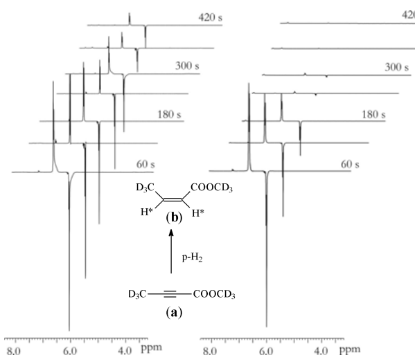
Figure 1: ^1\text{H} -NMR PHIP signals of ( b ) at increasing time intervals; the samples were kept at earth field ( 50 \mu\text{T} , left) and 0.1 \mu\text{T} (right).
