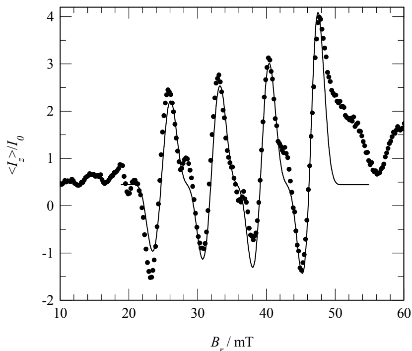
Figure: \text{CH}_3 tunnel resonance displaying DNP in \text{Cu}^{2+} doped zinc acetate
